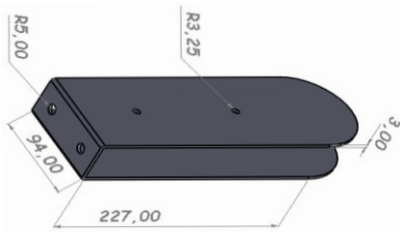
Wall Profile Falnges Duvar Flanşı 227 x 94x 3mm
