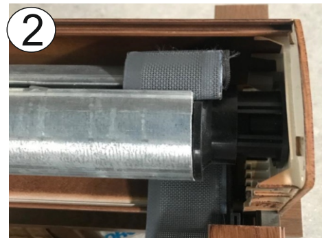
When the ribbon arrive to the motors place to the shaft
