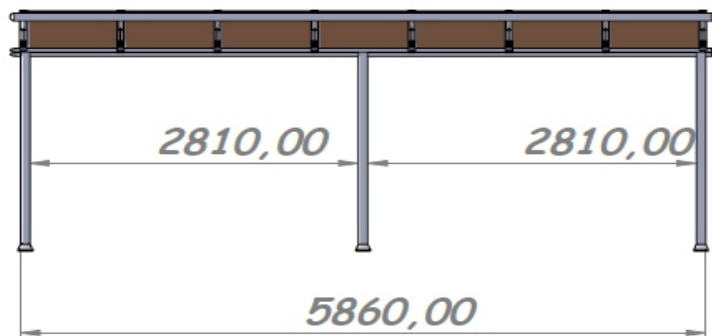
FRONT WIEW
